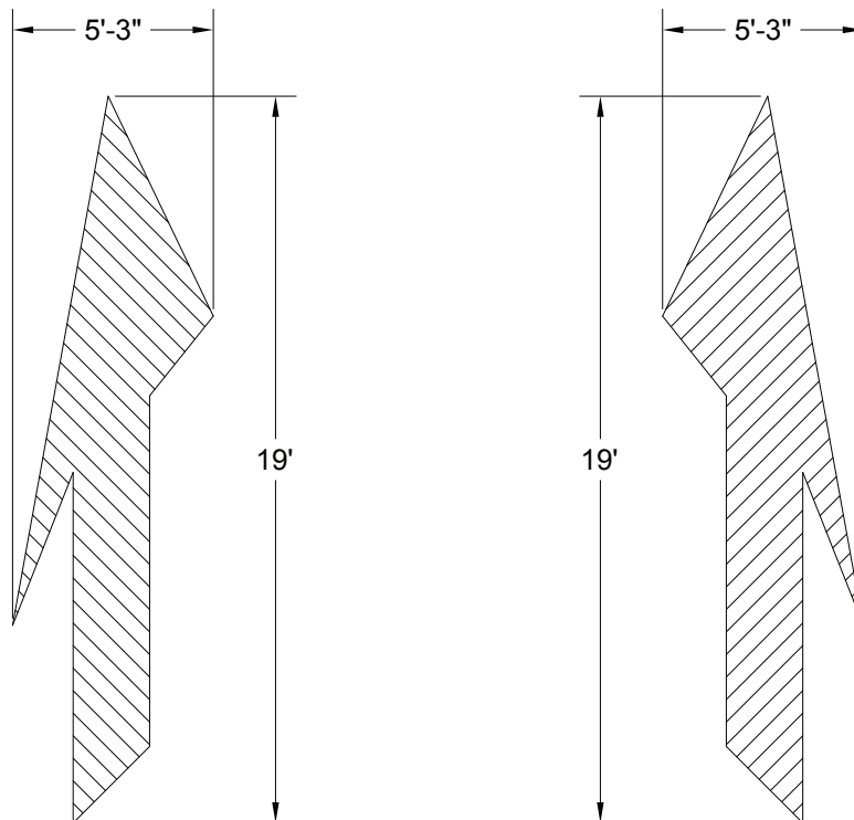
RIGHT LANE DROP ARROW
