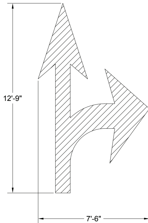
RIGHT TURN COMBO
