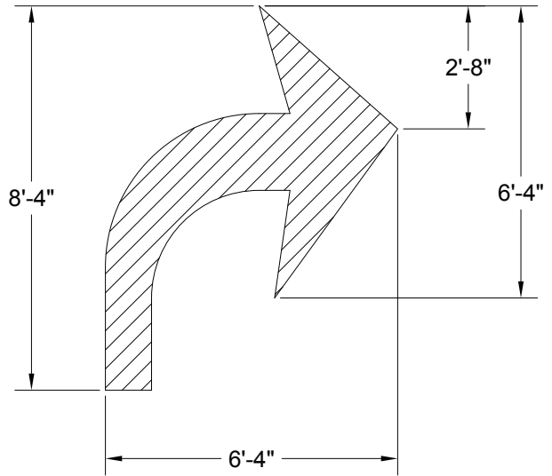
RIGHT TURN ARROW
